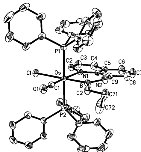
Figure 2. Molecular structure of 3 (ORTEP) in the crystal. Selected bond lengths [Å] and angles [°]: Os–B 2.072(3), Os–Cl 1.843(3), Os–N1 2.235(2), Os–Cl 2.6022(7), Os–P1 2.3799(7), Os–P2 2.3755(7), B–O2 1.401(4), B–N2 1.439(4); C1–Os–B 86.45(12), C1–Os–N1 174.50(10), C1–Os–Cl 93.19(8), N1–Os–B 88.05(10), N1–Os–Cl 92.31(6), P1–Os–P2 176.86(2), Cl–Os–B 179.31(8), B–N2–C9 132.2(2), Os–N1–C10 127.61(17), Os–B–O2 121.2(2), Os–B–N2 123.5(2).
